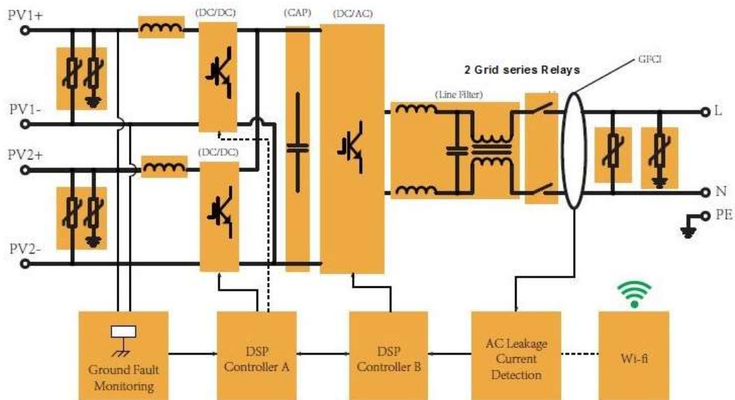
Models BLD-3K-TL3; BLD-3.5K-TL3 and BLD-4K-TL3, BLD-5K-TL3
